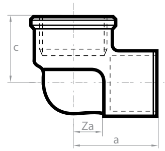
Female Elbow 90°
