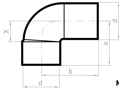
Street Elbow 90° - MF
