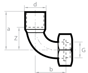
Bent Tap Connector 90°
