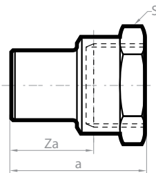
Straight male adaptor
