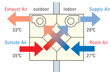
Principle of operation (heat exchanging)
